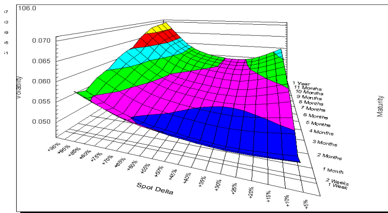
EURUSD Call Vol 5-95delta
